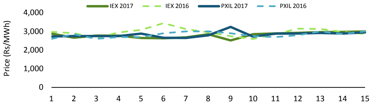
Year-on-year price comparison of power traded on IEX and PXIL (1-15 April)
